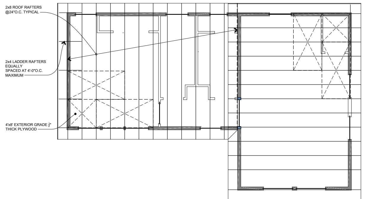
ROOF/CEILING FRAMING PLAN
