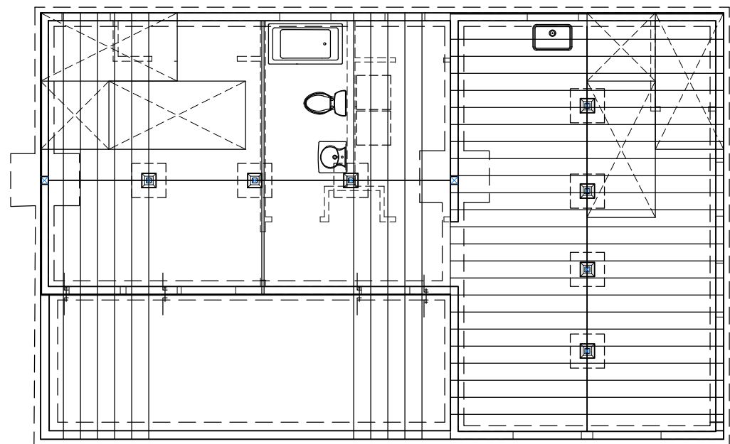
FLOOR FRAMING AND FOUNDATION PLAN
